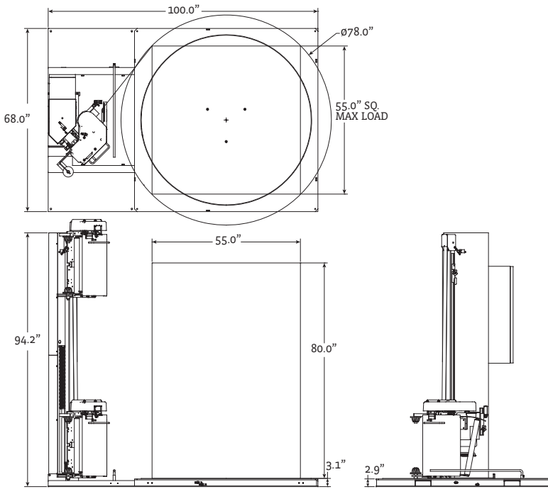
Flex LPD - Dimensions - Inches
