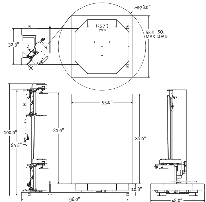
Flex HPD - Dimensions - Inches
