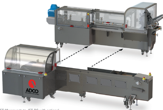
* JET-60 converts to JET-BC with optional auto-load barrel cam conversion shown here
